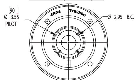
ZF184 (500009)
