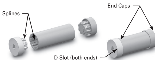
Figure 2 - Shaft Coupling
