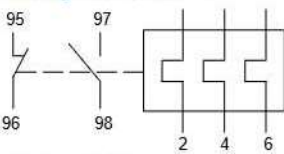
Typical IEC Wiring Schematic
