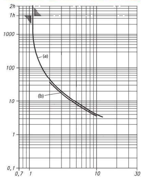
Cat. Nos. 193-T1AB48...AC25 Overload Relays
