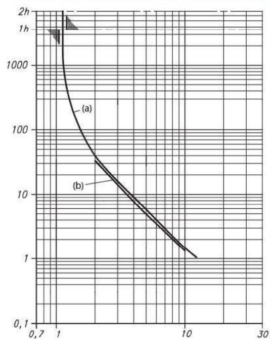
Cat. Nos. 193-T1BC30...BC38 Overload Relays
